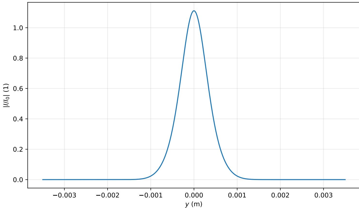
Intensity profile I(x = 0, y, z = 0.796)/I_0 , P_{in}=0.6P_{cr} , artificial time
